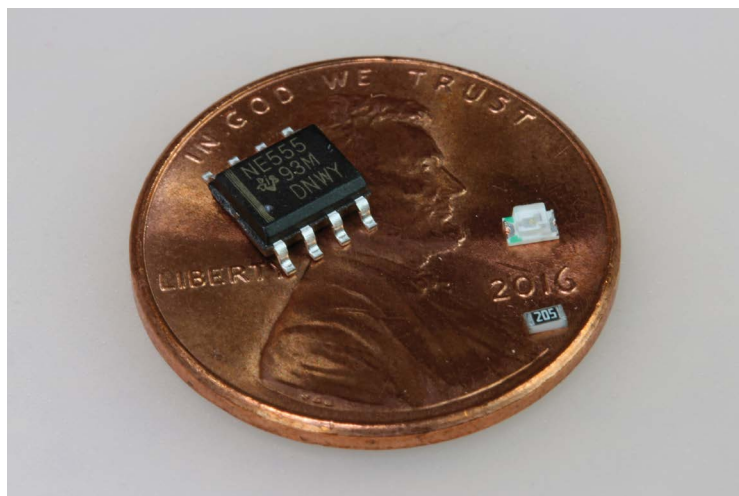
FIGURE 5-13: The size of SMT components
