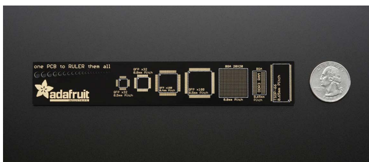
FIGURE 5-6: The front of the "One PCB to Ruler Them All"
