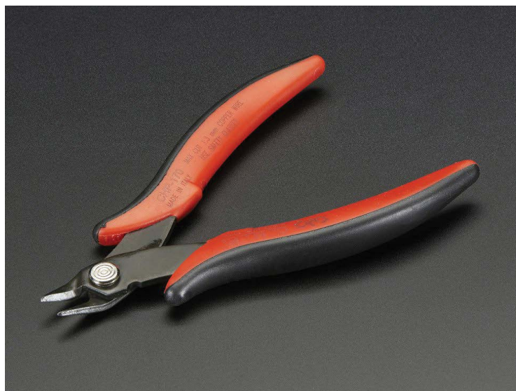
FIGURE 2-19: Diagonal flush cutting pliers are the best choice for hobby electronics. IMAGE COURTESY OF ADAFRUIT INDUSTRIES, CC BY-NC-SA 2.0.
